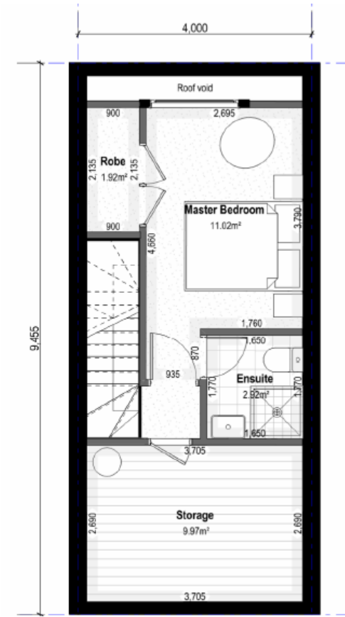
3 Type A Second Floor Plan 1:50
