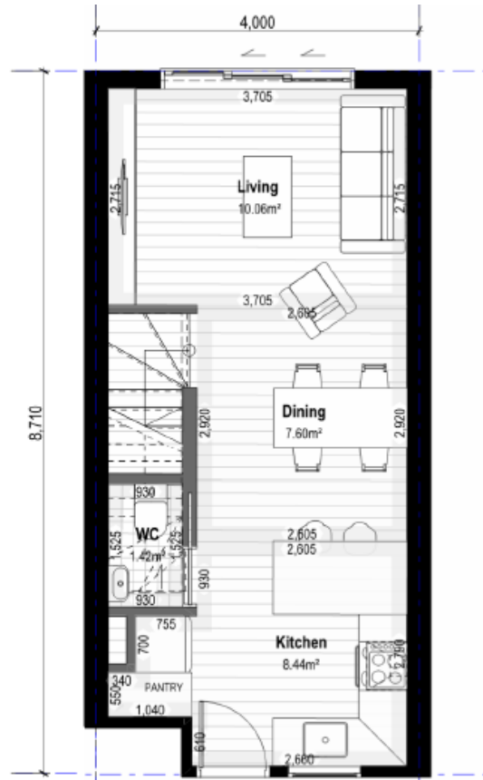
1 Type A Ground Floor Plan 1:50
